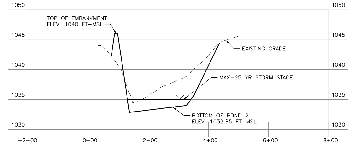
D POND 2 SECTION D IIII-H-C-18 0 100 200 SCALE IN FEET (HORIZONTAL) 0 5 10 SCALE IN FEET (VERTICAL)
