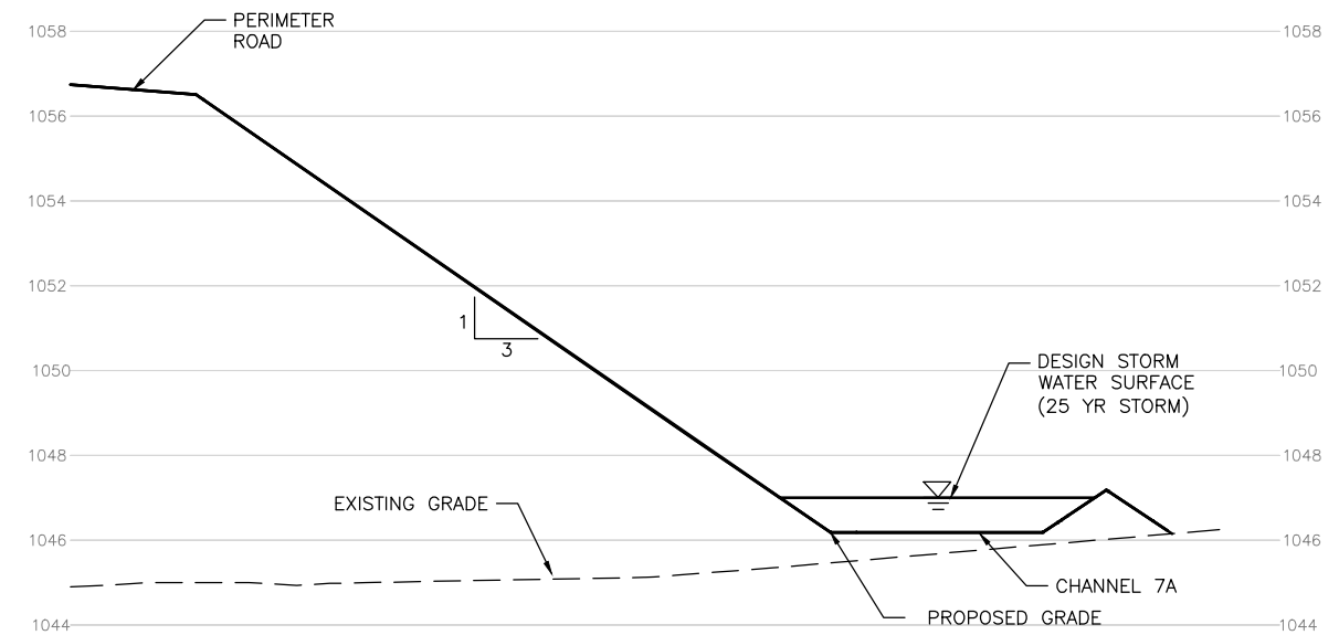
B SECTION 0 5 10 SCALE IN FEET (HORIZONTAL) 0 2.5 5 SCALE IN FEET (VERTICAL)
