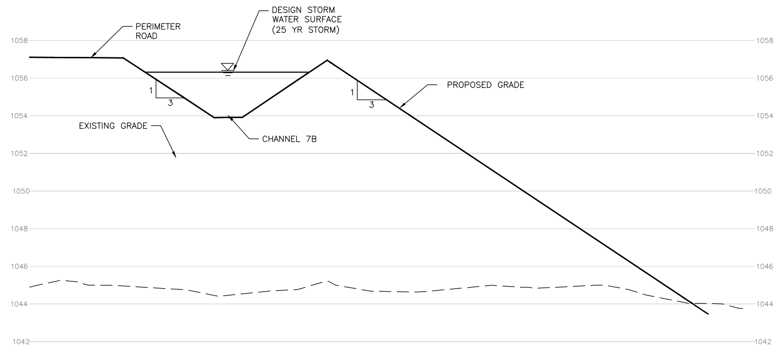
B SECTION SCALE IN FEET (HORIZONTAL): 0, 5, 10 SCALE IN FEET (VERTICAL): 0, 2.5, 5
