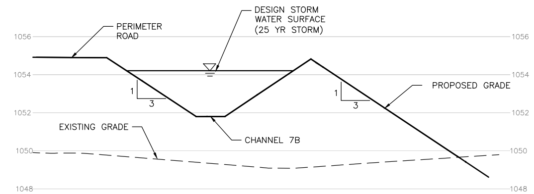
B SECTION SCALE IN FEET (HORIZONTAL): 0, 5, 10 SCALE IN FEET (VERTICAL): 0, 2.5, 5
