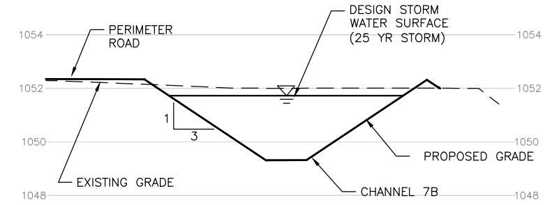
A SECTION SCALE IN FEET (HORIZONTAL): 0, 5, 10 SCALE IN FEET (VERTICAL): 0, 2.5, 5
