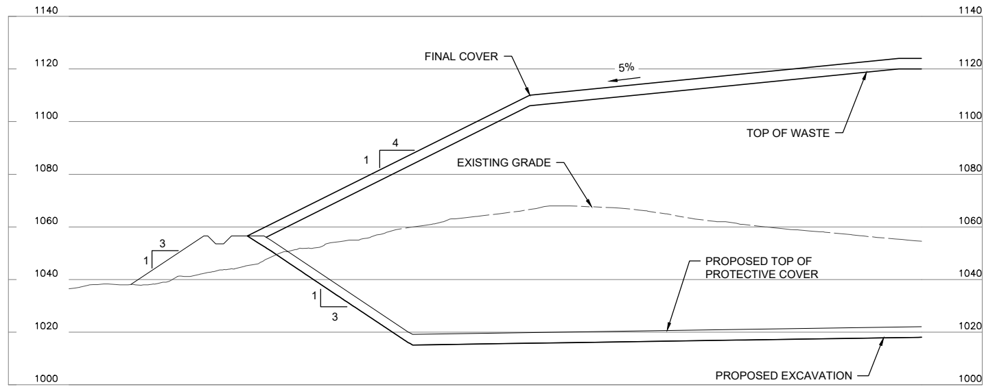
C FINAL COVER SECTION IILL-A-5 HORZ 0 50 100 VERT 0 5 10 SCALE IN FEET
