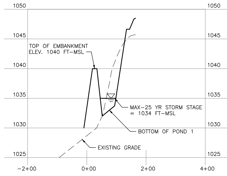
C POND 2 SECTION C IIII-H-C-18 0 100 200 SCALE IN FEET (HORIZONTAL) 0 5 10 SCALE IN FEET (VERTICAL)
