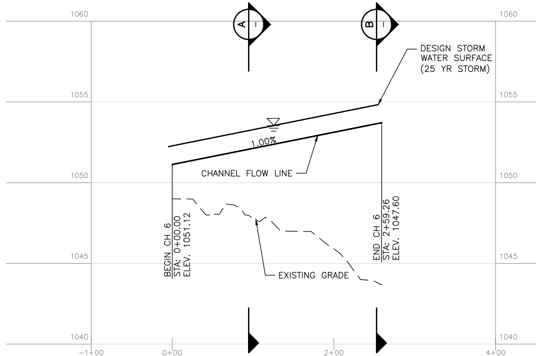
CH6 CHANNEL 6 PROFILE IIIH-C-4 SCALE IN FEET (HORIZONTAL) SCALE IN FEET (VERTICAL)
