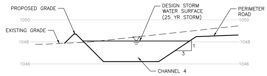
SECTION A SCALE IN FEET (HORIZONTAL) 0 5 10 SCALE IN FEET (VERTICAL) 0 2.5 5
