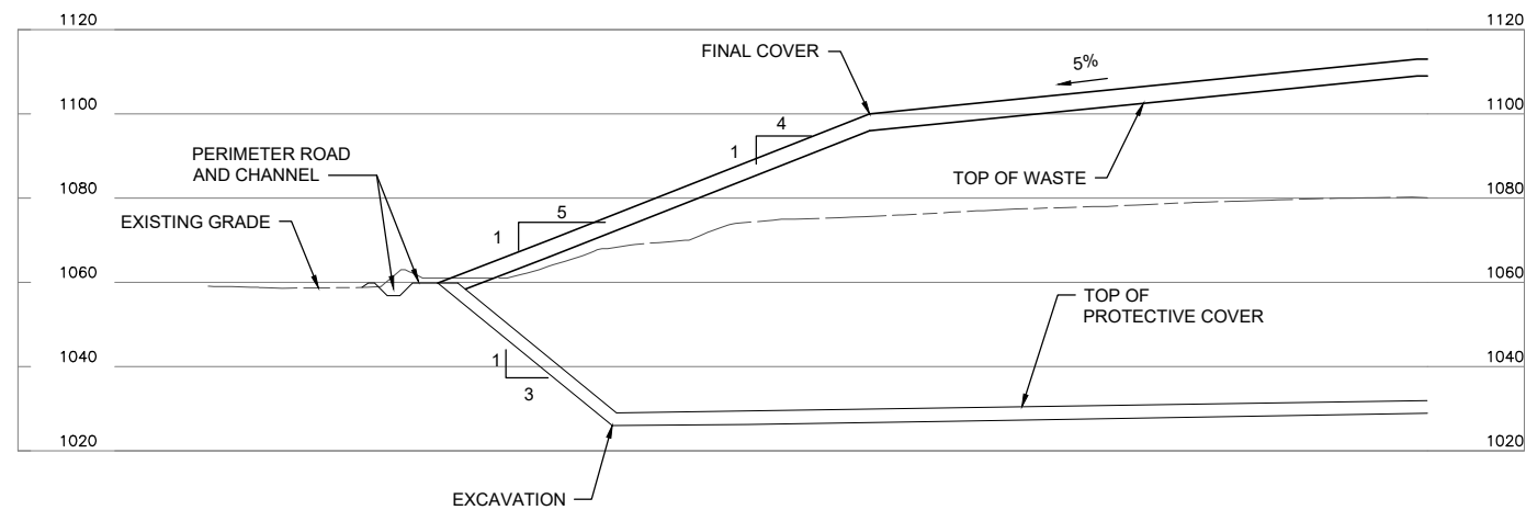
D FINAL COVER SECTION IILL-A-5 HORZ 0 50 100 VERT 0 5 10 SCALE IN FEET
