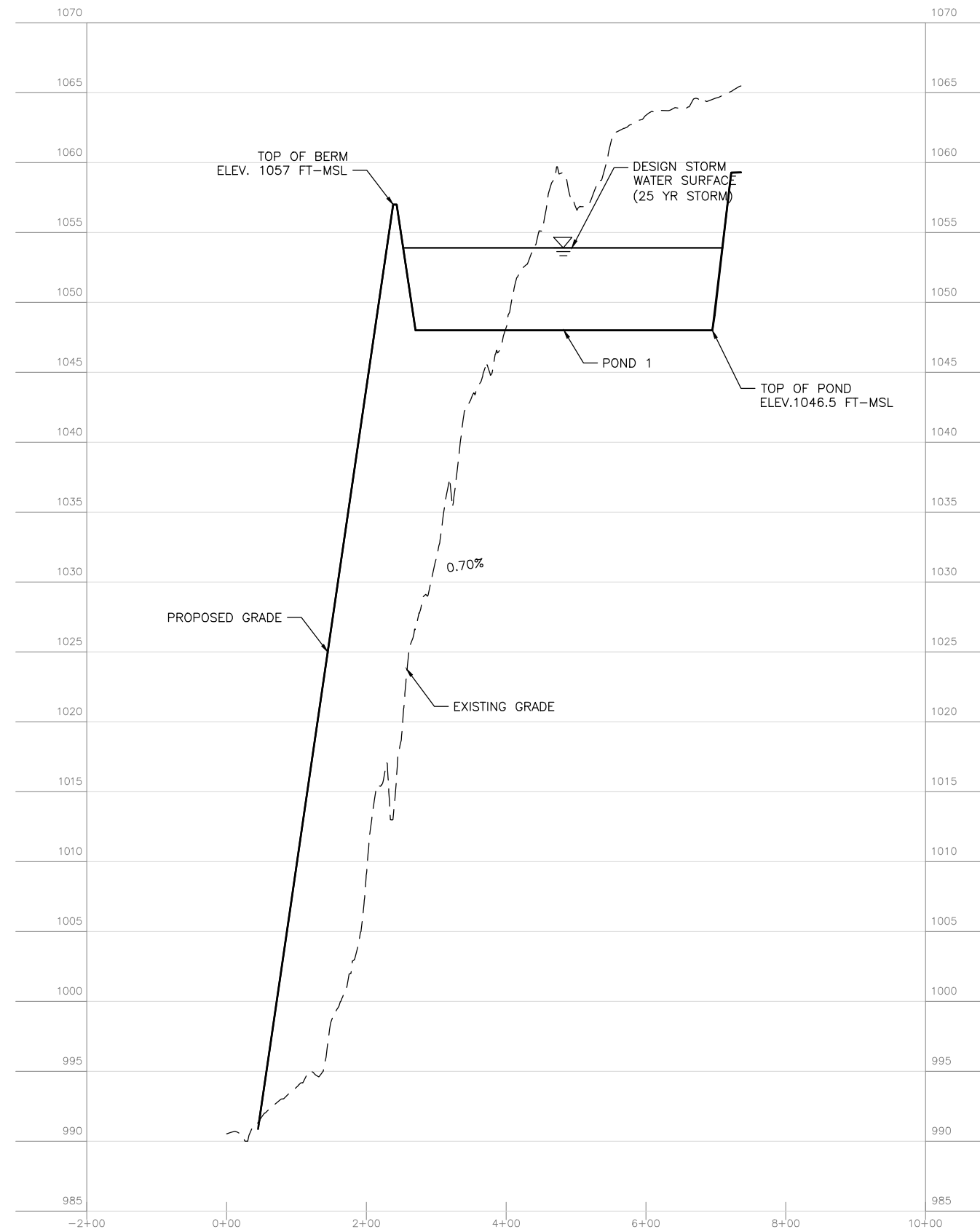
P1 IIIH-C-17 POND 1 SECTION 0 100 200 SCALE IN FEET (HORIZONTAL) 0 5 10 SCALE IN FEET (VERTICAL)
