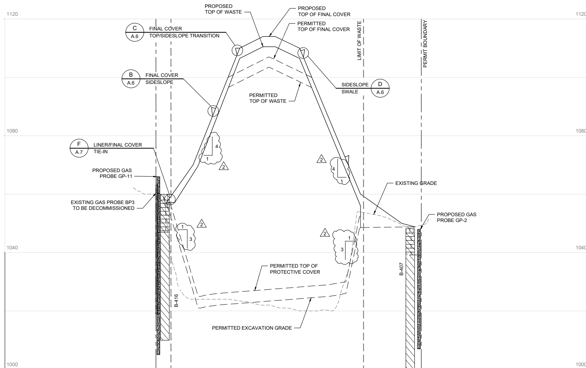
SECTION A B.2 HORIZ 0 100 200 VERT 0 10 20 SCALE IN FEET
