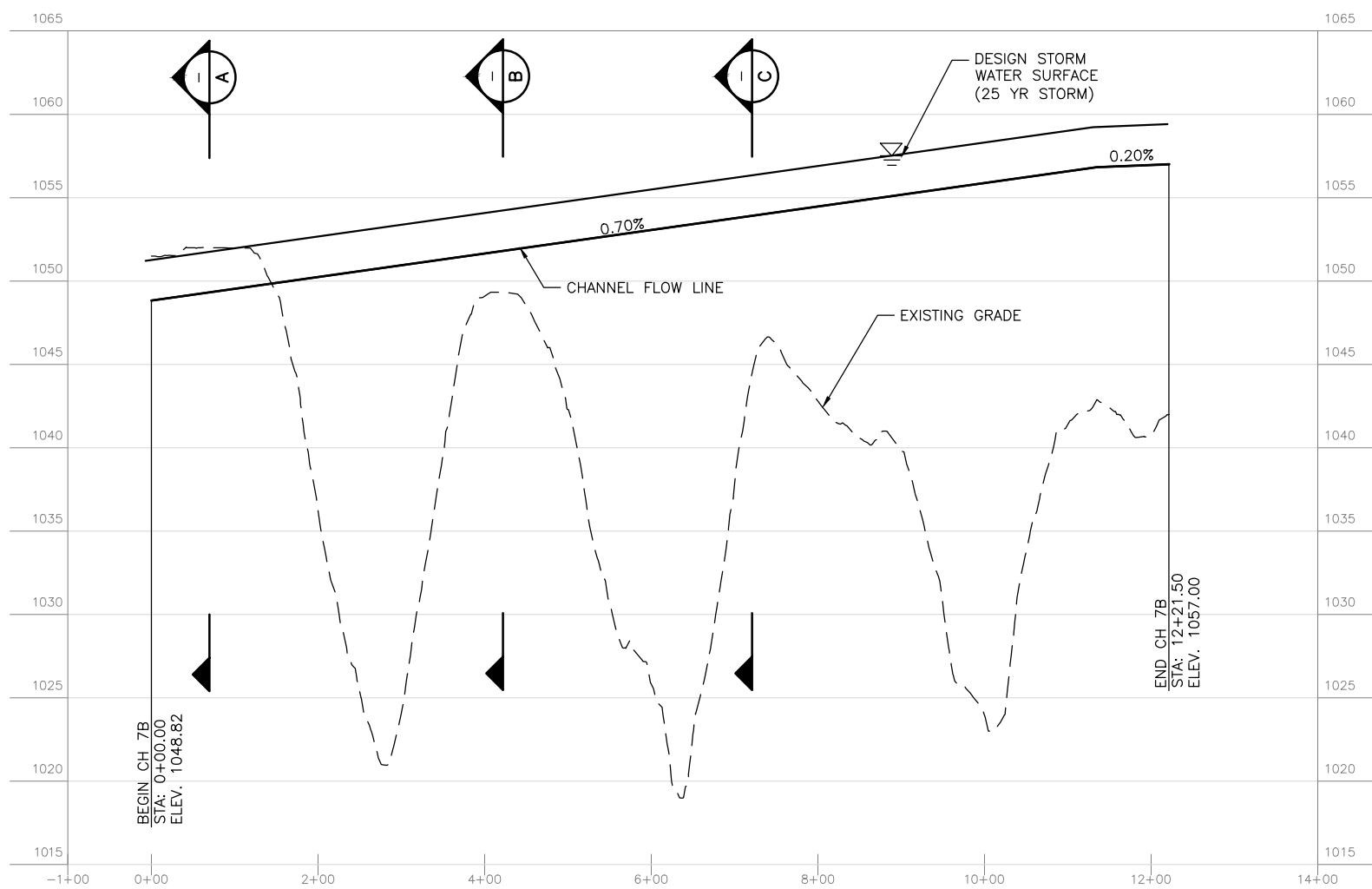
CH7B CHANNEL 7B PROFILE IIIH-C-11A SCALE IN FEET (HORIZONTAL): 0, 100, 200 SCALE IN FEET (VERTICAL): 0, 5, 10
